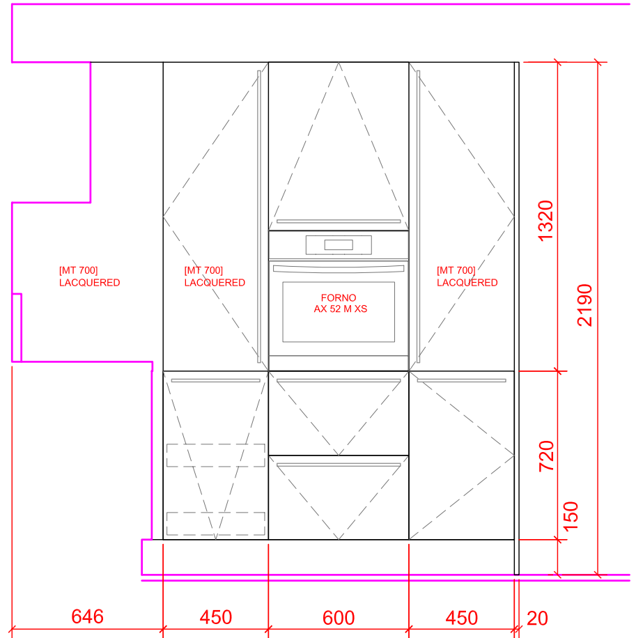
ELEVATION C
