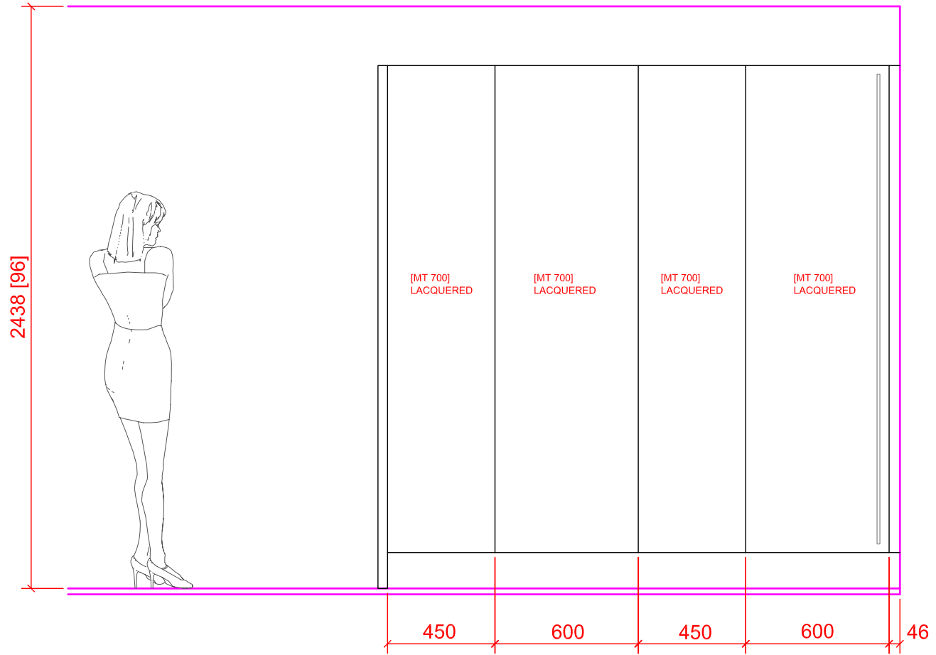
ELEVATION D
